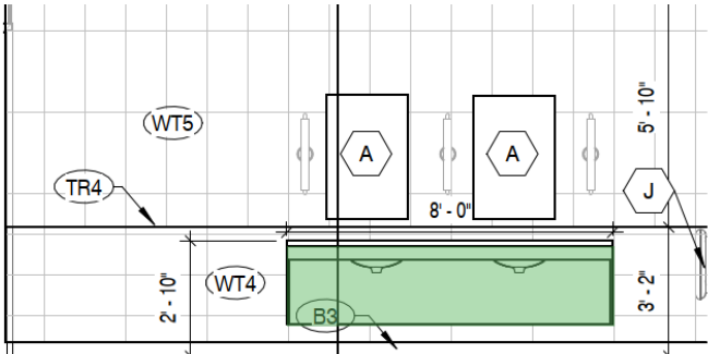
11 MENS RESTROOM RIGHT ELEVATION 1/4" = 1'-0"
