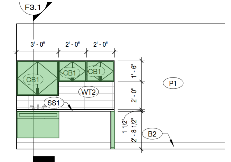
1 EXAM ROOM 1 FRONT ELEVATION 1/4" = 1'-0"
